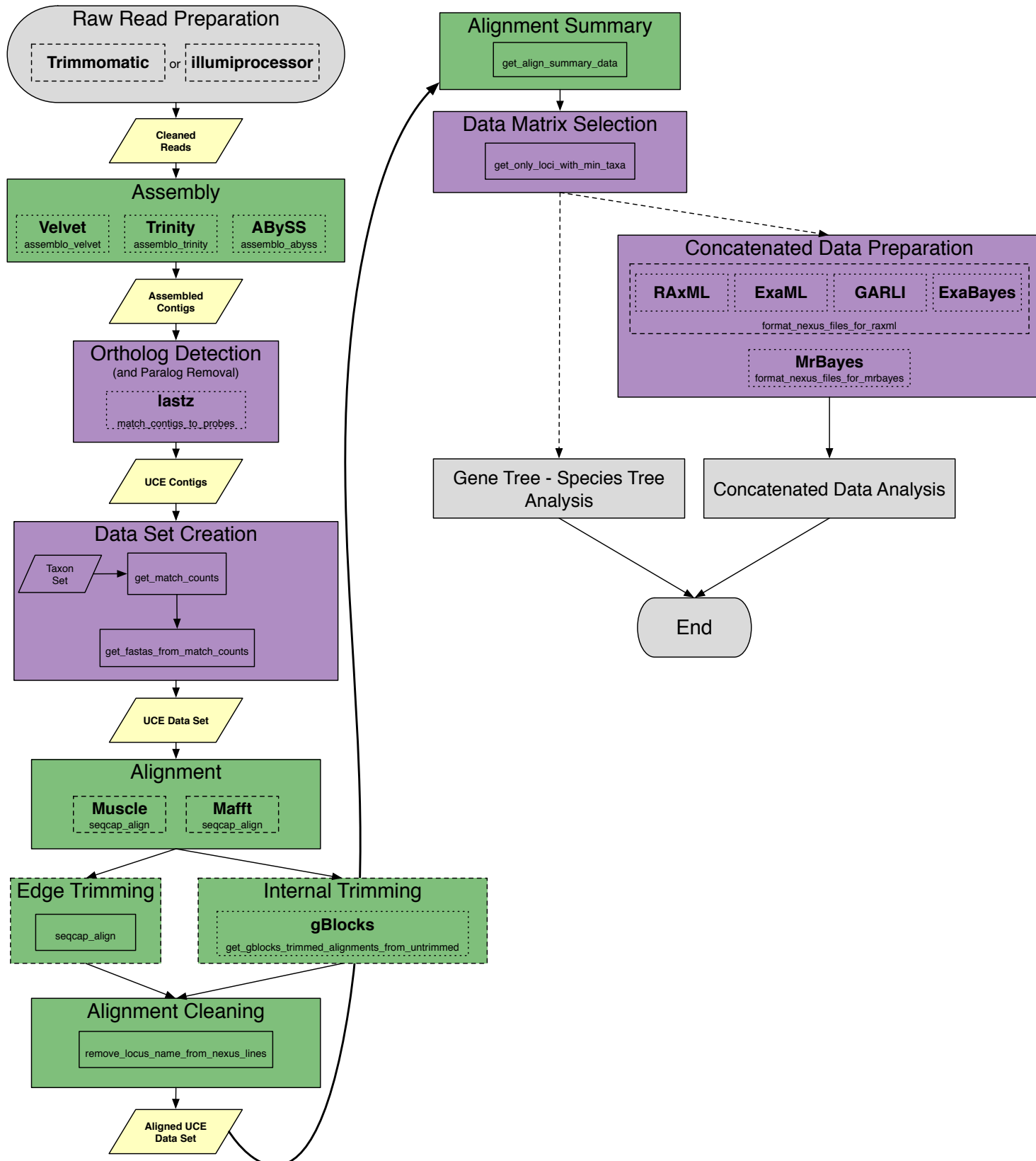
Supplementary Figure 1. PHYLUCE workflow for phylogenomic analyses of data collected from conserved genomic loci using targeted enrichment.
